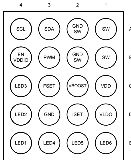
Figure 2. Bottom View
